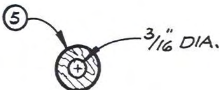
ARM SPACER 1/8" THICK PLYWOOD (2 REQ'D)
